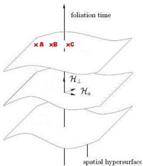
Fig. 1. The above plot shows the (3 + 1)-decomposition of a four-dimensional spacetime. Spatial hypersurfaces are stacked together along a foliation parameter. The components of the Hamiltonian tangential and perpendicular to the hypersurfaces are shown (but note that there are actually three components tangential to the hypersurfaces).
